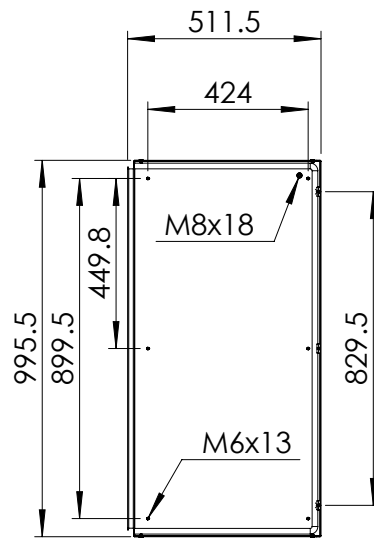
Inside left door view
