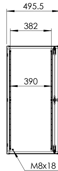
Inside right door view
