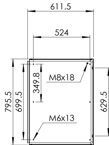
Inside left door view
