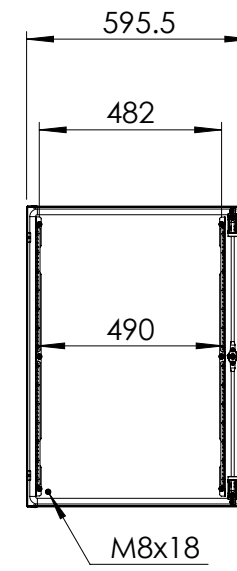
Inside right door view
