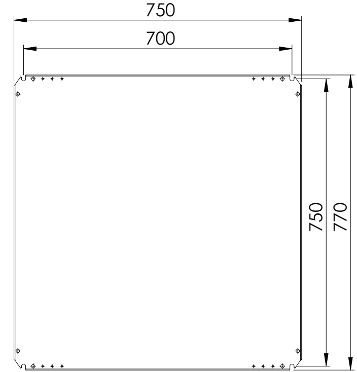
Mounting plate
