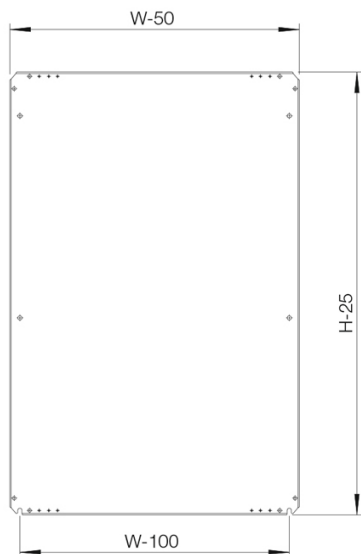
Mounting plate
