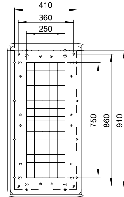
Inside enclosure view
