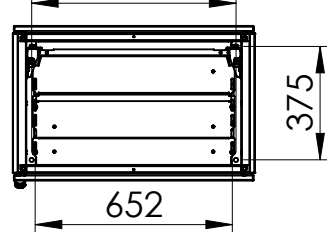
Sectional top view (without bottom plates)
