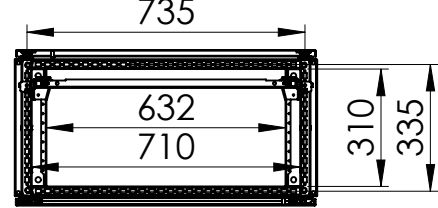
Sectional top view (without bottom plates)
