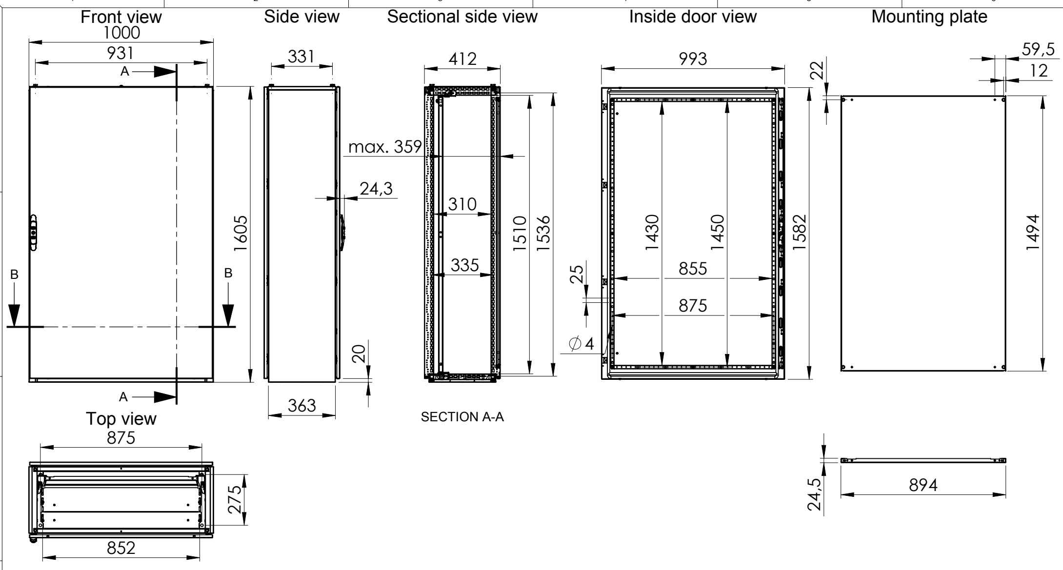
Sectional top view (without bottom plates)
