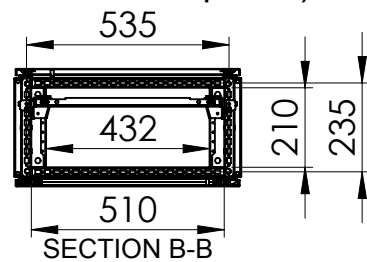
Sectional top view (without bottom plates)
