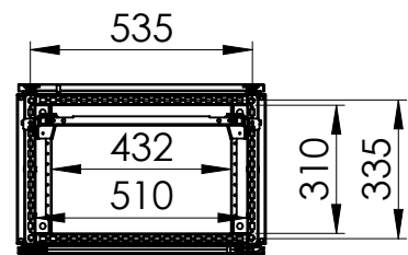
Sectional top view (without bottom plates)
