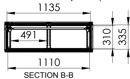
Sectional top view (without bottom plates)
