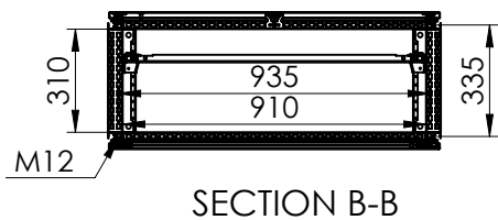
Sectional top view (without bottom plates)
