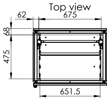
Sectional top view (without bottom plates)
