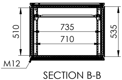
Sectional top view (without bottom plates)
