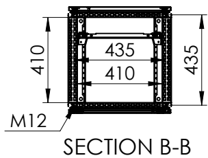
Sectional top view (without bottom plates)
