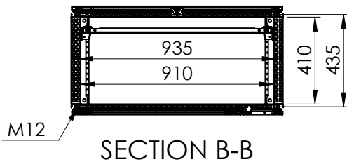
Sectional top view (without bottom plates)
