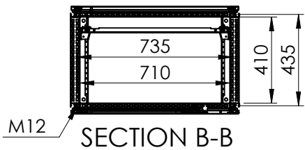
Sectional top view (without bottom plates)
