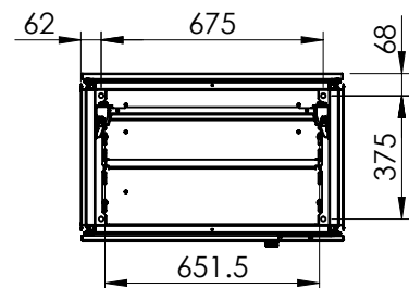
Sectional top view (without bottom plates)
