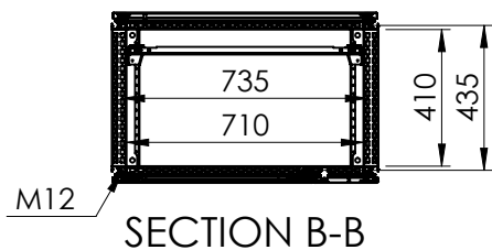
Sectional top view (without bottom plates)
