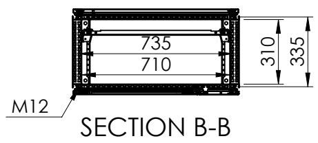
Sectional top view (without bottom plates)
