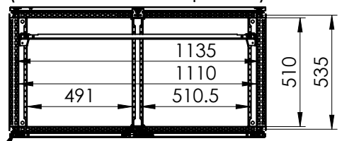
Sectional top view (without bottom plates)
