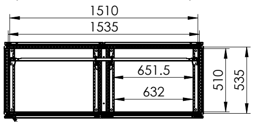
Sectional top view (without bottom plates)
