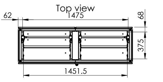
Sectional top view (without bottom plates)
