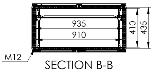
Sectional top view (without bottom plates)
