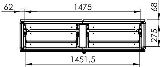
Sectional top view (without bottom plates)
