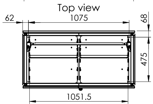
Sectional top view (without bottom plates)
