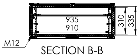
Sectional top view (without bottom plates)
