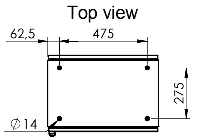
Sectional top view (without bottom plates)
