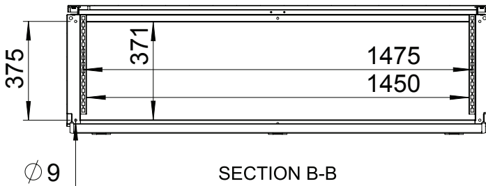
Sectional top view
