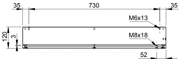
Sectional top view
