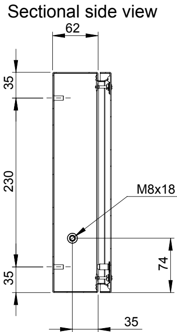
Section B-B
