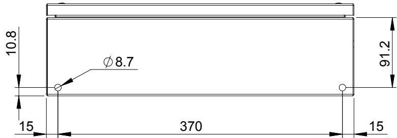
Bottom view
