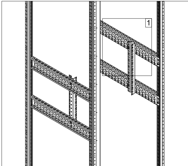
600 wide enclosure
