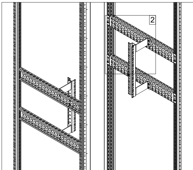
800 wide enclosure
