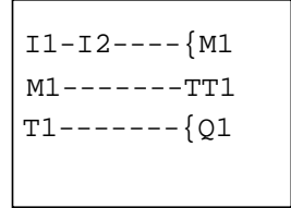
Pico-Schaltplan
